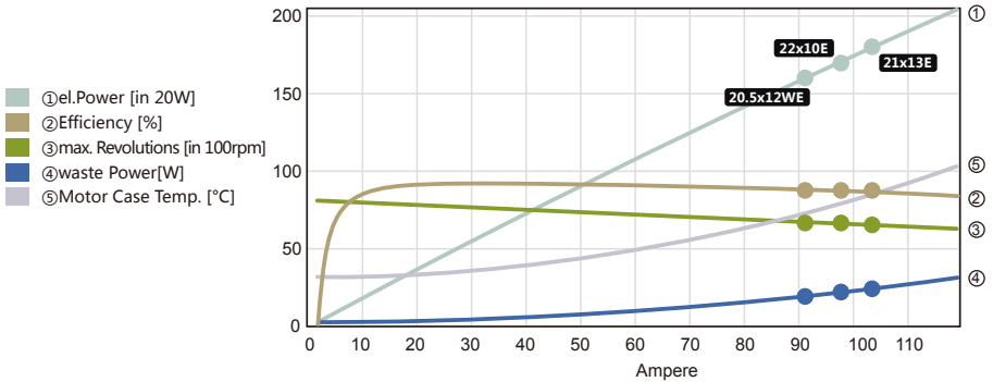
Motor Characteristics
